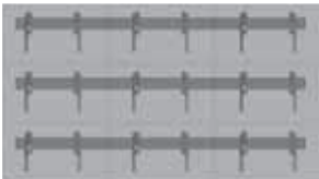
3 x 3 solution
