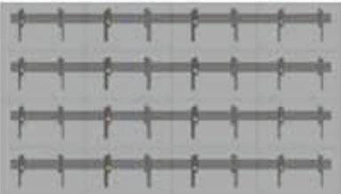
4 x 4 solution
