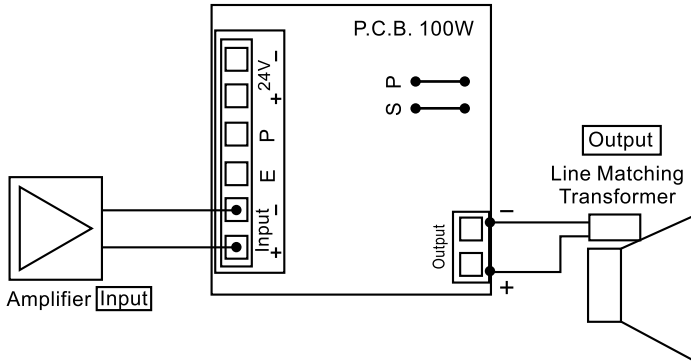
Standard System
