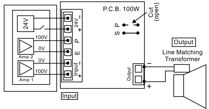
4 Wire System Emergency message from another amplifier
