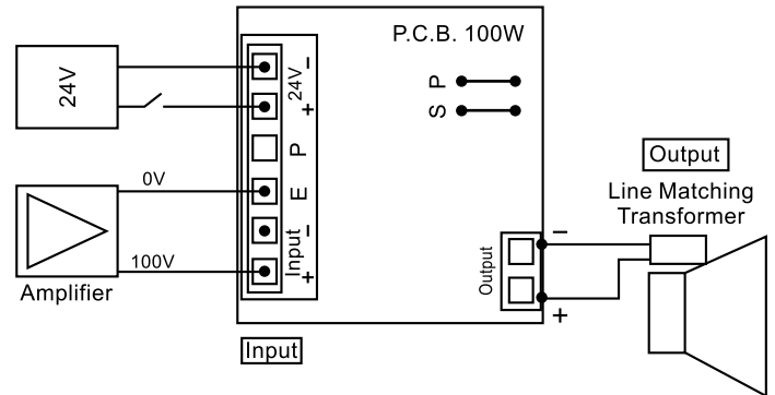
4 Wire System Emergency message from same amplifier
