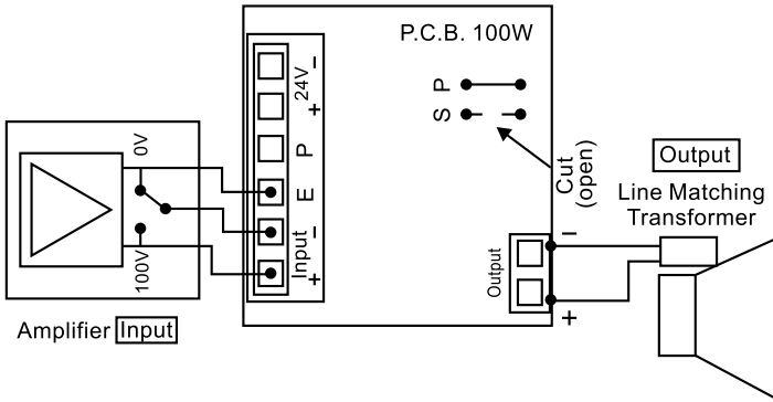
3 Wire System
