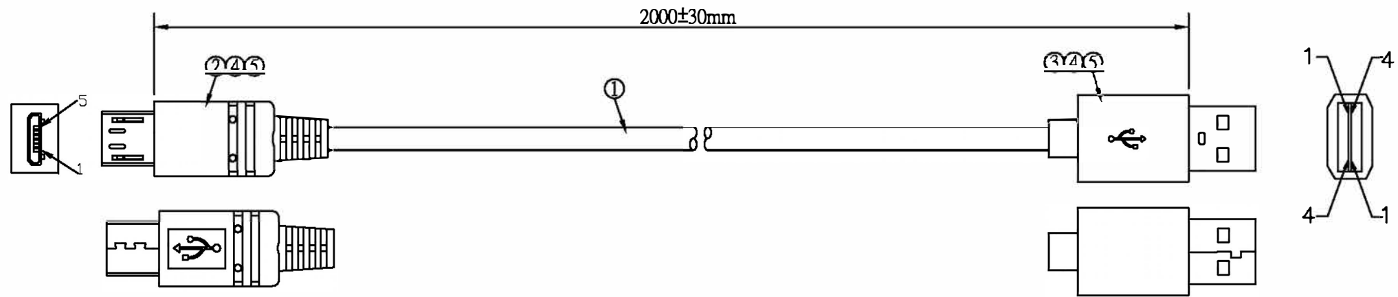
MICRO USB BM(Nickel plated) Transparent molding No.:186
