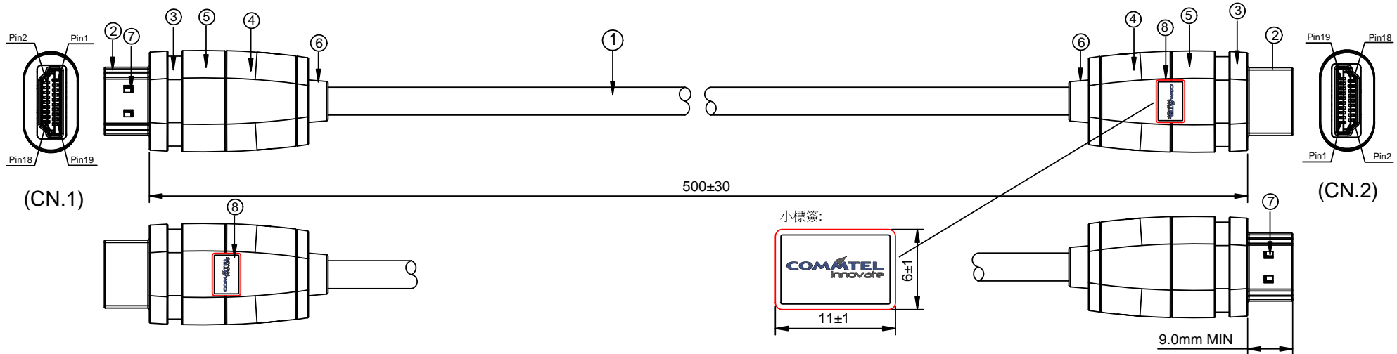
(A).Wire Pin Assignment and Wire Description.
